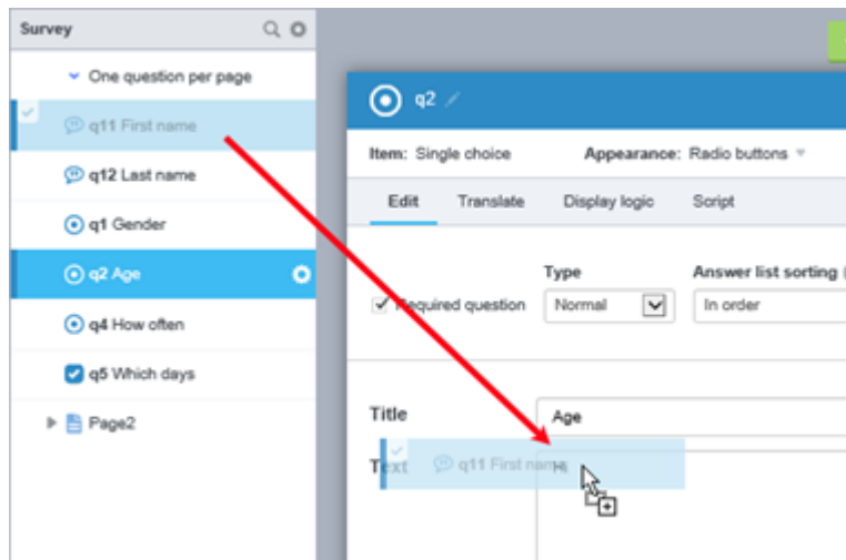
Figure 136 Dragging and dropping one question into another
